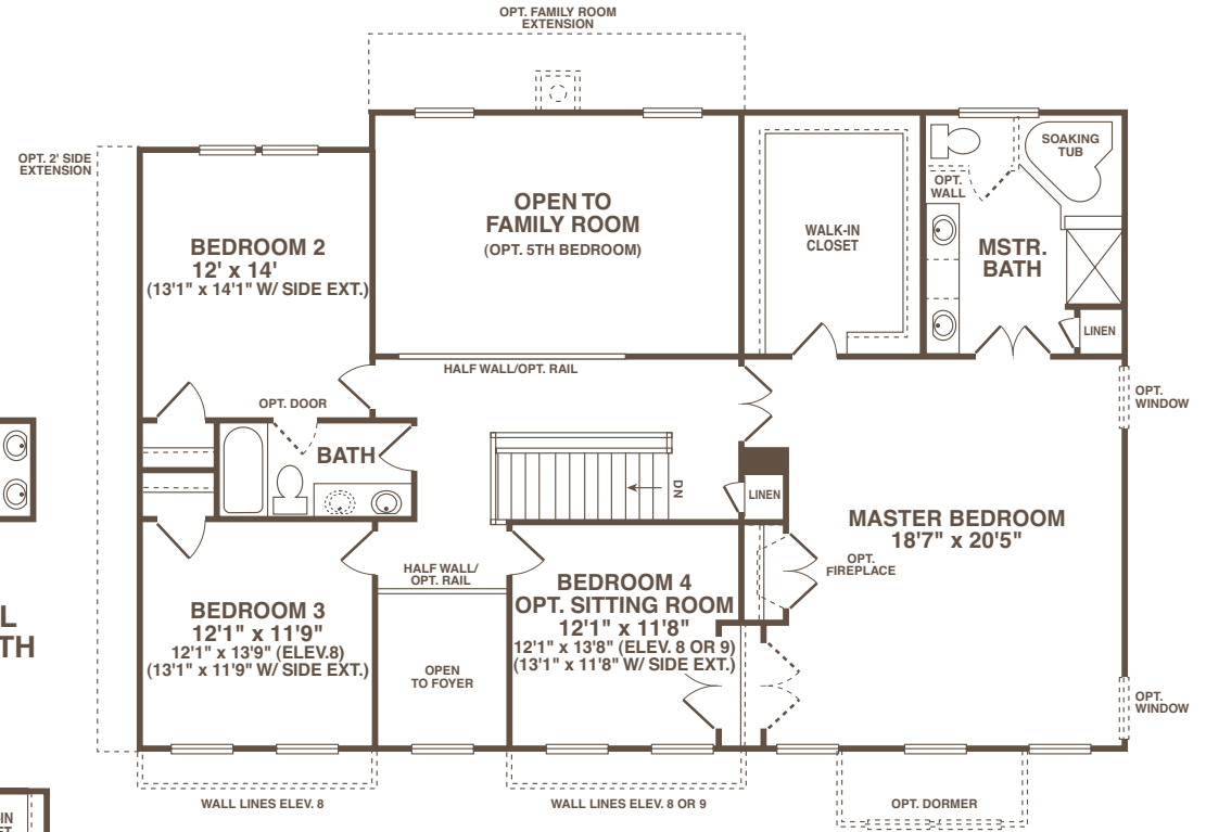
DELUXE SECOND FLOOR PLAN
