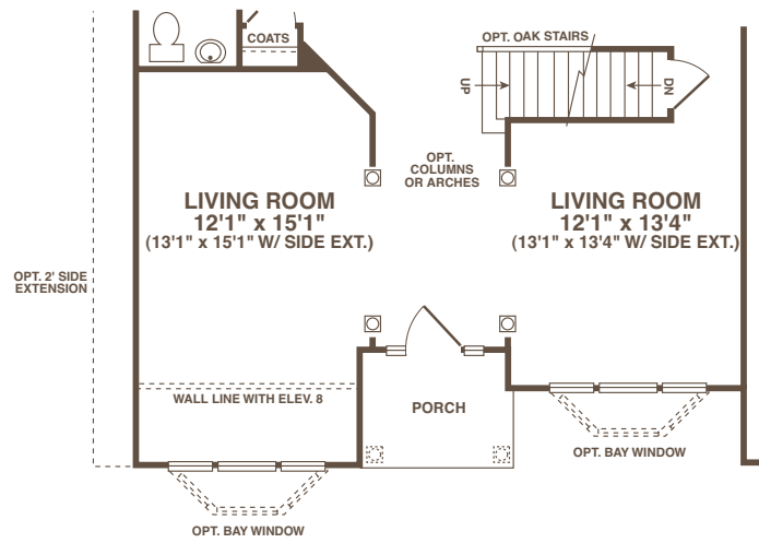
LIVING ROOM/DINING ROOM FRONT EXTENSION OPTIONS ELEVATIONS 6, 9 AND 10
