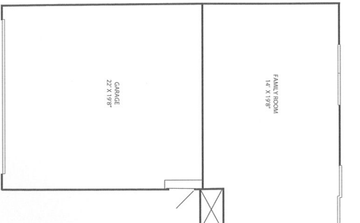
OPT. FIRST FLOOR W/ 2 CAR GARAGE
